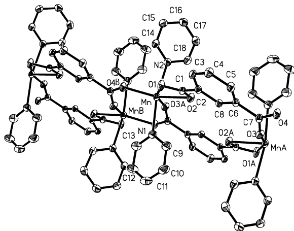
Fig. 1. ORTEP diagram of 1 showing the atom-numbering scheme of a Mn(m-phth)(py)_2 moiety and thermal ellipsoids at 30% probability. Mn_2(\mu-COO)_2 and Mn_2(\mu-isophthalate)_2 moieties alternately link to form one-dimensional chain of complex 1 .
