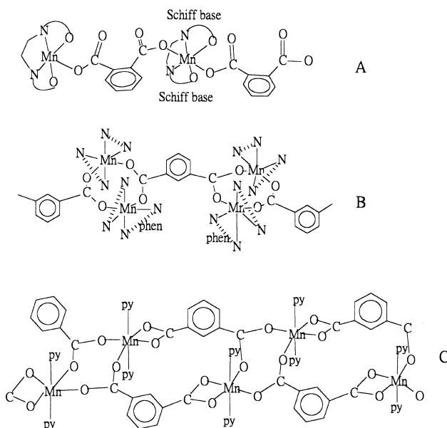
Scheme 1. (A) Single phthalate bridges between Mn moieties of N_2O_2 Schiff base. (B) Single phthalate bridges between (phen)_2Mn moieties. (C) Double phthalate bridges between (py)_2Mn moieties.
